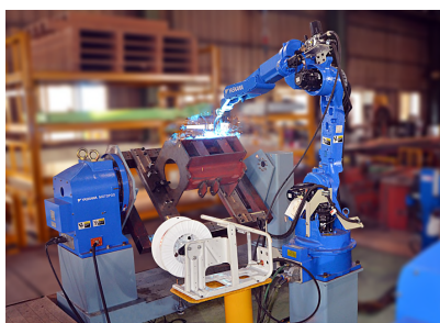
▲ 彈性機械手臂銲接系統 Multi-function Robotic Arm Welding System
